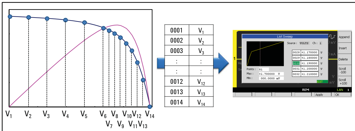
Figure 3. The B2900A Series' list sweep mode makes it easy to characterize photovoltaic cells in the region of interest
